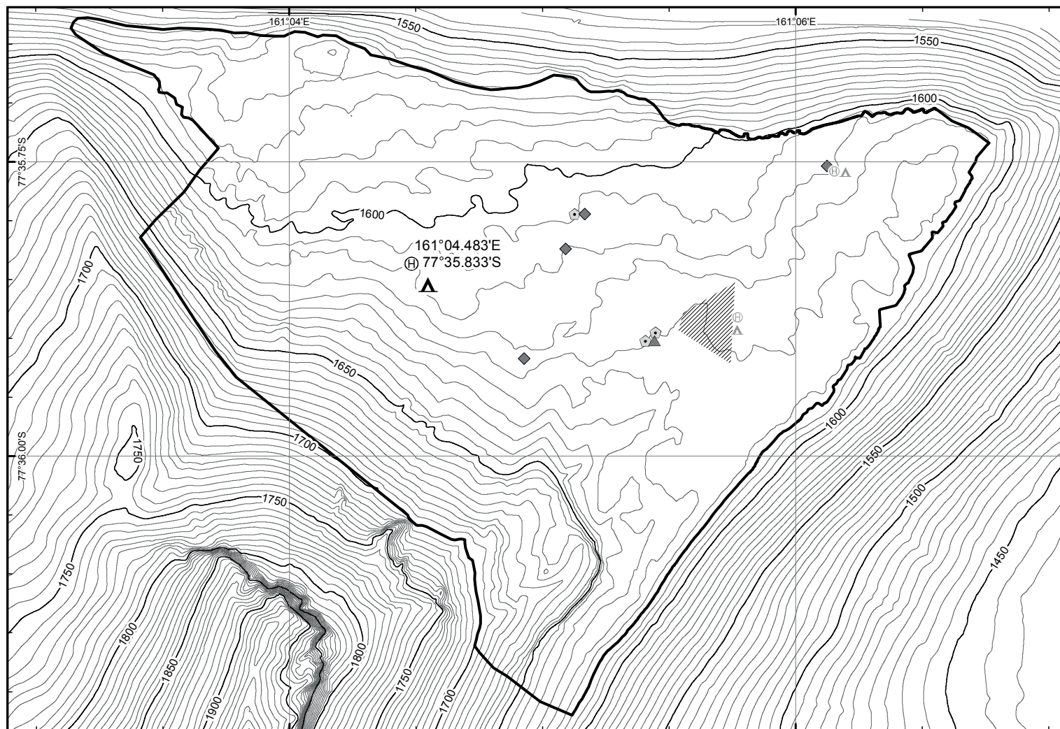
Map 2: ASPA No. 138: Linnaeus Terrace, topography and boundary
