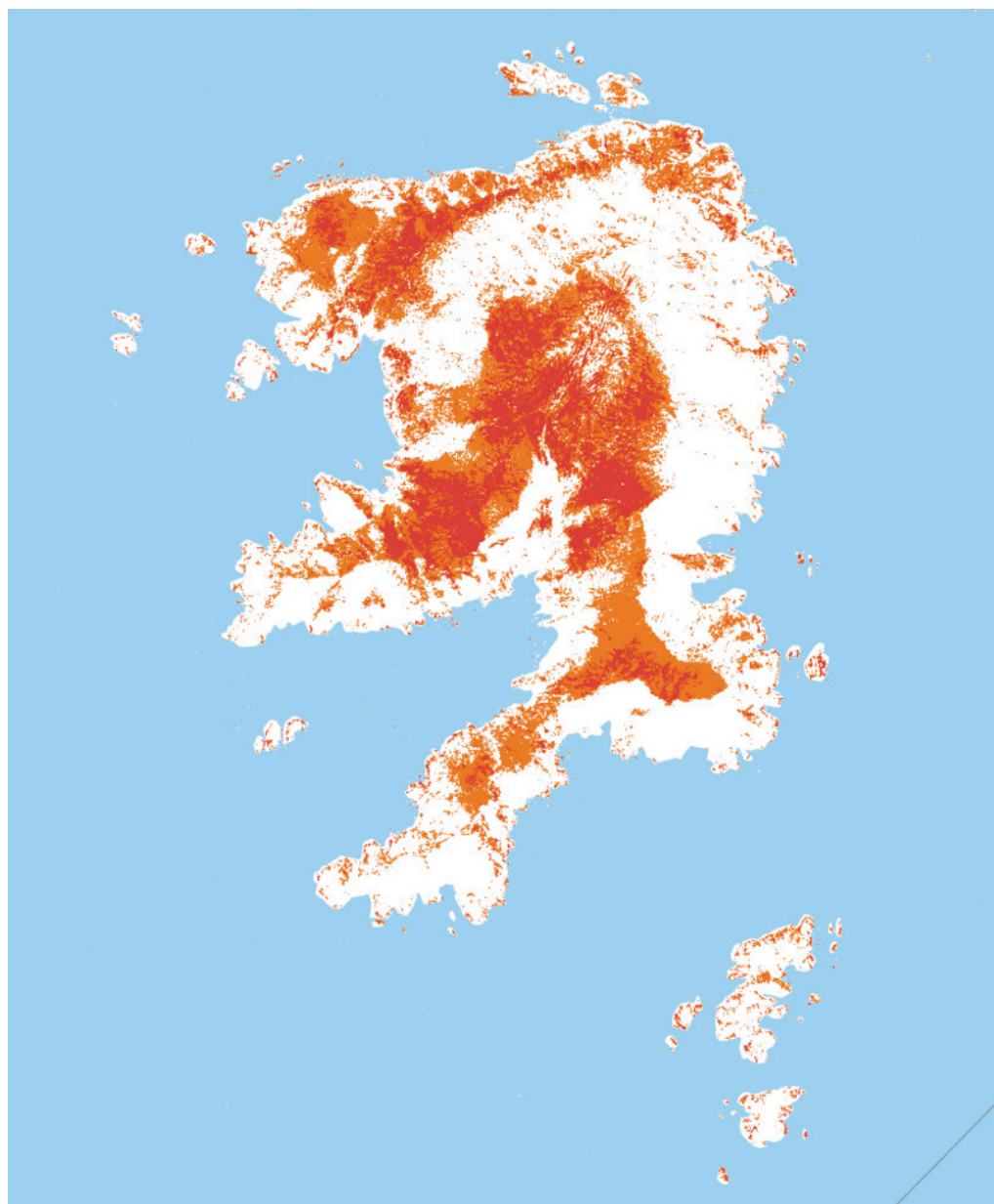
Figure 4. Normalised Difference Vegetation Index (NDVI), derived from satellite imagery, for ASPA No. 109 Moe Island, South Orkney Islands, showing vegetation cover using a colour scale of white orange red, with red indicating the highest NDVI values.
