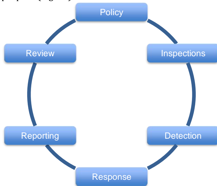
Figure 11. Biosecurity cycle
